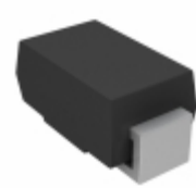
SMAJ48C-E3/5A Electro-Films (EFI) / Vishay TVS DIODE 48V 85.5V DO214AC
