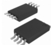
CAT24C08YI-GT3JN ON Semiconductor IC EEPROM 8KBIT 400KHZ 8TSSOP
