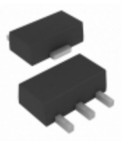
MCP1703AT-1202E/MB Microchip Technology IC REG LDO 1.2V 0.2A SOT89-3
