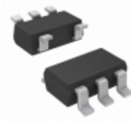
MCP1316MT-33LE/OT Microchip Technology IC SUPERVISOR 3.3V SOT23-5
