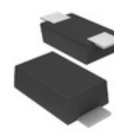
KDZLVTFR91 Rohm Semiconductor DIODE ZENER 91V 1W SOD123FL
