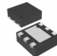
RT9081A-13GQZA(2) Richtek USA Inc. IC LDO 0.5A LOW DROPOUT ZADFN-6
