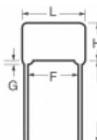
ECQ-P1H391JZ3 Panasonic Electronic Components CAP FILM 390PF 5% 50VDC RADIAL
