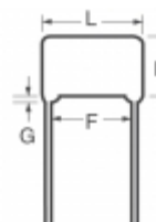
ECQ-P1H333GZ3 Panasonic Electronic Components CAP FILM 0.033UF 2% 50VDC RADIAL
