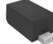
CDZVT2R11B Rohm Semiconductor DIODE ZENER 11V 100MW VMN2M
