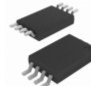
BR24C02-10TU-2.7 Rohm Semiconductor IC EEPROM 2KBIT 400KHZ 8TSSOP
