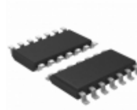
NLVHC02ADR2 ON Semiconductor IC GATE NOR 4CH 2-INP 14-SOIC
