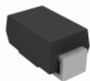
P4SMA9.1CA-E3/5A Electro-Films (EFI) / Vishay TVS DIODE 7.78V 13.4V DO214AC
