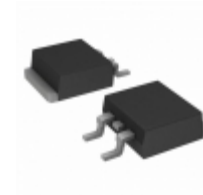
IRL3714ZSPBF Infineon Technologies MOSFET N-CH 20V 36A D2PAK
