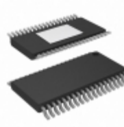
LTC3865EFE#TRPBF ADI (Analog Devices, Inc.) IC REG CTRLR BUCK 38TSSOP
