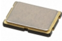
CX5Z-A1B2C5-40-24.0D18 Cardinal Components Inc. CRYSTAL 24.0000MHZ 18PF SMD
