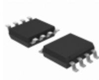
11LC020-E/SN Microchip Technology IC EEPROM 2KBIT 100KHZ 8SOIC
