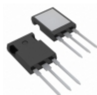
IXFR80N15Q IXYS MOSFET N-CH 150V 75A ISOPLUS247
