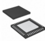
PIC18F46K80-E/ML Microchip Technology IC MCU 8BIT 64KB FLASH 44QFN
