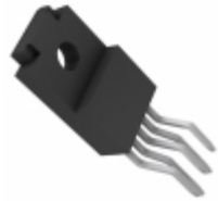
BA033ST-V5 Rohm Semiconductor IC REG LDO 3.3V 1A TO220FP-5
