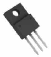
BA7808CP-E2 Rohm Semiconductor IC REG LDO 8V 1A TO220CP-3
