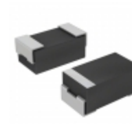
CWR29KH336KBHB AVX Corporation CAP TANT 33UF 10% 25V 2915
