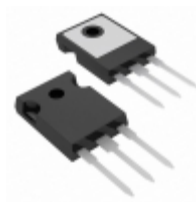
IRFP350PBF Electro-Films (EFI) / Vishay MOSFET N-CH 400V 16A TO-247AC
