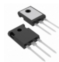
IRFP350LCPBF Vishay Siliconix MOSFET N-CH 400V 16A TO-247AC
