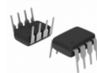
PAA132 IXYS Integrated Circuits Division RELAY OPTOMOS 600MA DP-NO 8-DIP
