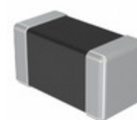
TMK042CG8R1DD-W Taiyo Yuden CAP CER 8.1PF 25V COG/NP0 01005
