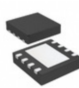
MCP4132T-502E/MF Microchip Technology IC RHEO DGTL SNGL 5K SPI 8DFN
