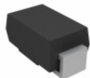
BYS10-35HE3/TR Electro-Films (EFI) / Vishay DIODE SCHOTTKY 35V 1.5A DO214AC
