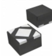
MIC5317-2.8YMT-T5 Microchip Technology IC REG LDO 2.8V 0.15A 4TDFN
