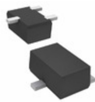
MA3S79500L Panasonic Electronic Components DIODE SCHOTTKY 30V 30MA SSMINI3
