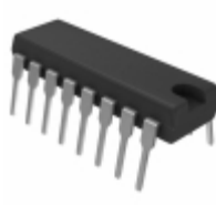
MAX520BEPE Maxim Integrated IC DAC QUAD SER 8BIT R/R 16-DIP
