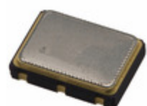
357LD5C040M0000 CTS-Frequency Controls OSC VCXO 40.000MHZ HCMOS TTL SMD
