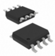
AO4850 Alpha & Omega Semiconductor Inc. MOSFET 2N-CH 75V 2.3A 8SOIC
