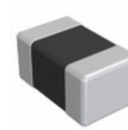
DFE201210U-1R0M=P2 Murata Electronics FIXED IND 1.0UH 2.0A 95MOHM
