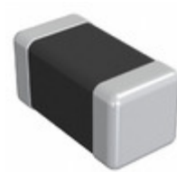
DFE18SAN1R0ME0L Murata Electronics FIXED IND 1UH 1.6A 144 MOHM SMD
