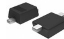
MM3Z39VC AMI Semiconductor / ON Semiconductor DIODE ZENER 39V 200MW SOD323F
