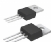
MJE15028G ON Semiconductor TRANS NPN 120V 8A TO220AB
