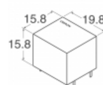
G5LA-1A4-CF DC5 Omron Electronics Inc-EMC Div RELAY GEN PURPOSE SPST 10A 5V
