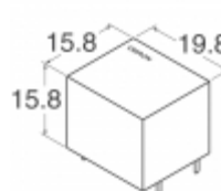
G5LA-1A4-CF DC24 Omron Electronics Inc-EMC Div RELAY GEN PURPOSE SPST 10A 24V
