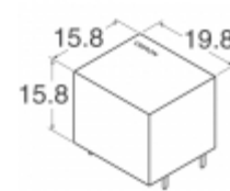
G5LA-1A4-CF DC9 Omron Electronics Inc-EMC Div RELAY GEN PURPOSE SPST 10A 9V
