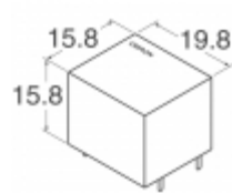
G5LA-1A4-CF DC12 Omron Electronics Inc-EMC Div RELAY GEN PURPOSE SPST 10A 12V
