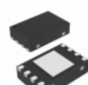
MCP6H82T-E/MNY Microchip Technology IC OPAMP GP 5.5MHZ RRO 8TDFN
