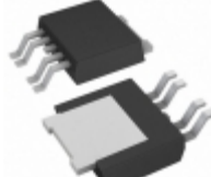
BD450M5WFPJ-CZE2 Rohm Semiconductor IC REG LDO 5V 0.5A TO-252-J5F
