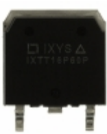
IXTT16P60P IXYS MOSFET P-CH 600V 16A TO-268
