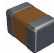
CDR01BP470BKZRAP Electro-Films (EFI) / Vishay CAP CER 47PF 100V BP 0805
