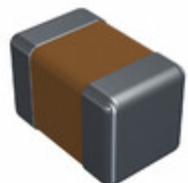
CDR01BP470BKZSAP Electro-Films (EFI) / Vishay CAP CER 47PF 100V BP 0805
