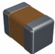
CDR01BP470BKZSAR Electro-Films (EFI) / Vishay CAP CER 47PF 100V BP 0805
