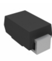
SMAJ110CA-M3/61 Vishay Semiconductor Diodes Division TVS DIODE 110VWM 177VC DO-214AC
