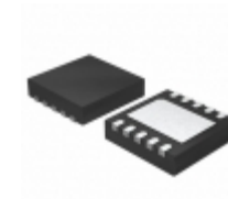
MCP4652T-103E/MF Microchip Technology IC DGTL POT 10K 257TAPS 10-DFN
