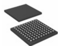
ATSAMS70N20B-CFN Micrel / Microchip Technology IC MCU 32BIT 1MB FLASH 100VFBGA
