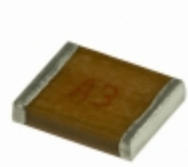
MC22FF152F-TF Cornell Dubilier Electronics (CDE) CAP MICA 1500PF 1% 1KV 2220
