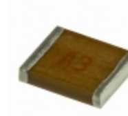
MC22FF152D-TF Cornell Dubilier Electronics (CDE) CAP MICA 1500PF 0.5% 1KV 2220
