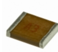
MC22FF161F-F Cornell Dubilier Electronics (CDE) CAP MICA 160PF 1% 1KV 2220
