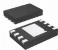
BR24G128NUX-3TTR Rohm Semiconductor IC EEPROM 128KBIT 400KHZ 8VSON
