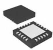
MCP4441T-104E/ML Microchip Technology IC DGTL POT 129TAPS QUAD 20QFN
