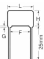
ECQ-P1H222GZ Panasonic Electronic Components CAP FILM 2200PF 2% 50VDC RADIAL
