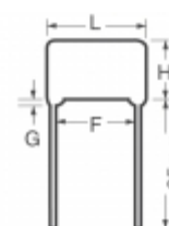
ECQ-P1H223GZ3 Panasonic Electronic Components CAP FILM 0.022UF 2% 50VDC RADIAL
