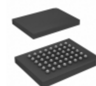
SST39VF402C-70-4I-B3KE Microchip Technology IC FLASH 4MBIT 70NS 48TFBGA
