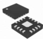
MAX4747ETE+ Maxim Integrated IC SWITCH ANLG QUAD SPDT 16TQFN
