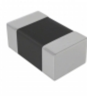
MLF2012E6R8MTD25 TDK Corporation FIXED IND 6.8UH 15MA 650 MOHM
