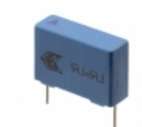
B32922C3154M000 EPCOS CAP FILM 0.15UF 20% 305VAC RAD
