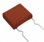
ECW-F2564HAB Panasonic Electronic Components CAP FILM 0.56UF 3% 250VDC RADIAL
